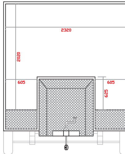
front elevation
