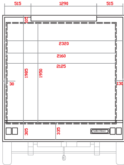
back elevation
